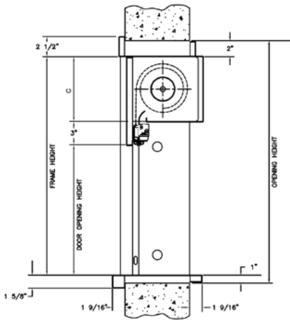
BETWEEN JAMBS UNIT (SLIP IN)
