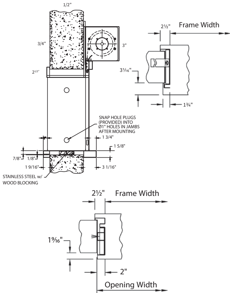
FACE MOUNTED (BUILT IN)
