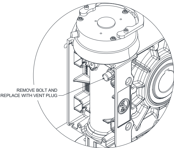
Figure 7.5 – Optional Wall Mounted APEX Pro Configuration
