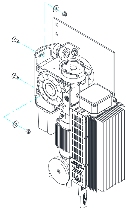
Figure 7.2.4 – Motor To Motor Bracket Mounting
