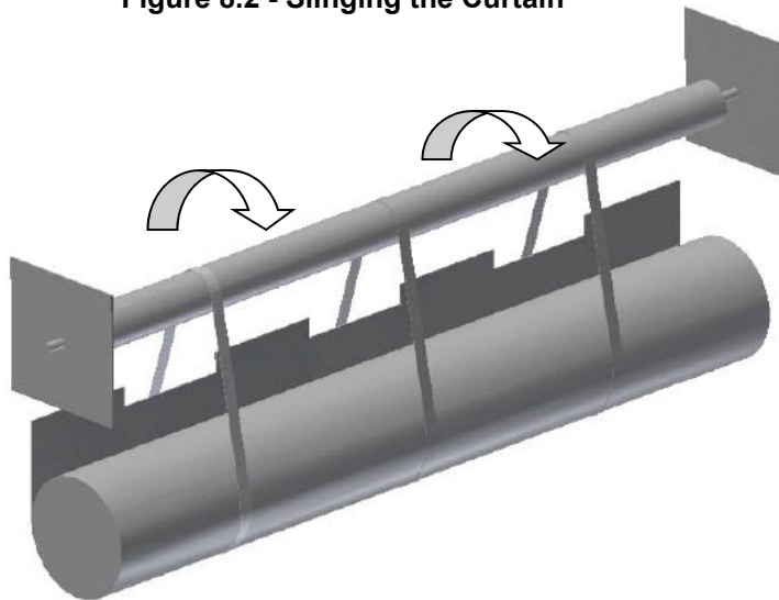
Figure 8.2 - Slinging the Curtain
