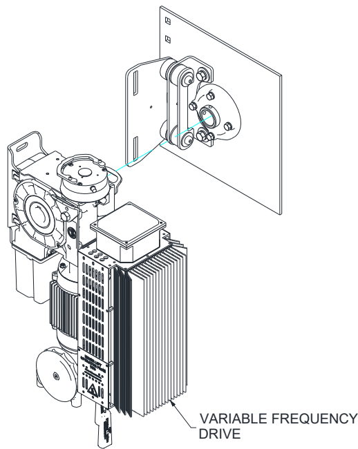
Figure 7.2.2 – Motor To Shaft Mounting
