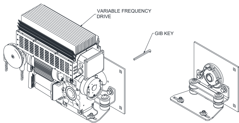
Figure 7.4 – Gearbox Housing Bolt Location
