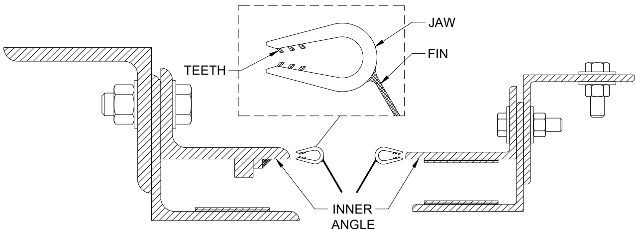
Figure A.1 – Guide Weather Seal
