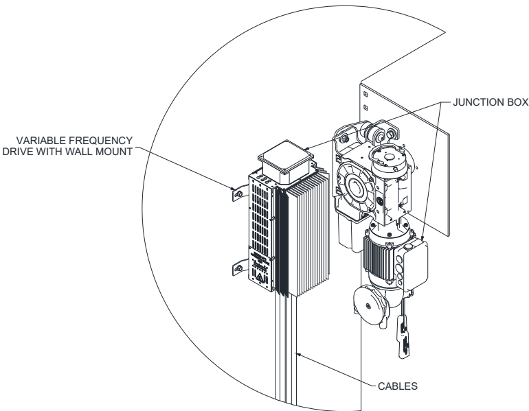
Figure 7.5 – Optional Wall Mounted APEX Pro Configuration
