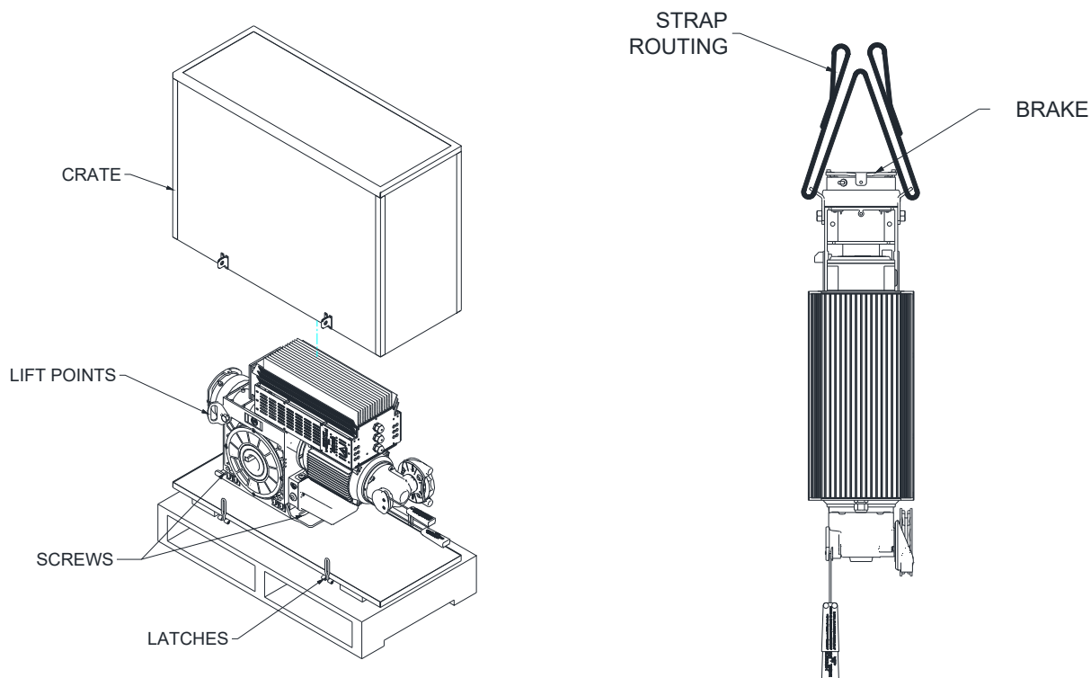
Figure 7.1 – Operator Lifting and Strap Routing
