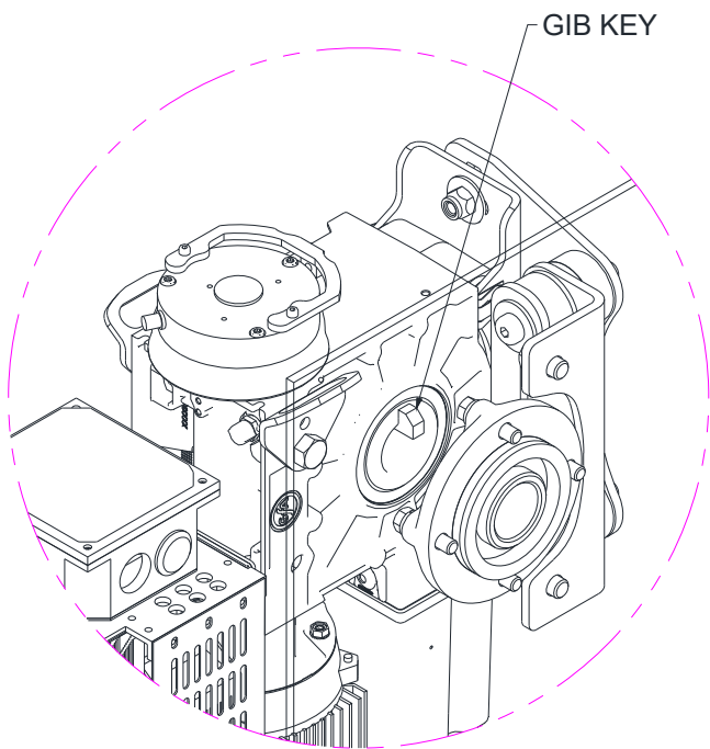
Figure 7.2.3 – Gib Key Orientation
